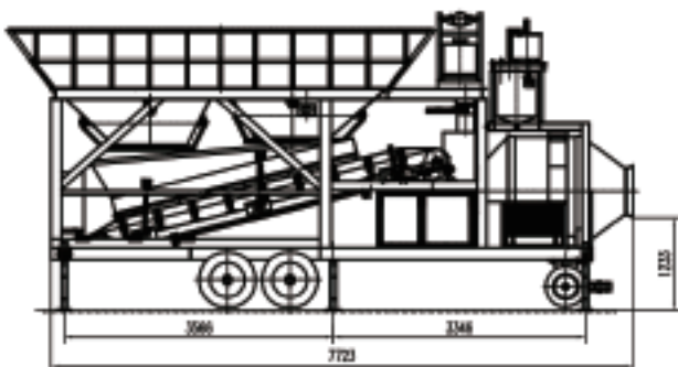
● Layout of portable concrete batching plant
