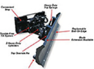
Six Way Dozer Blade
